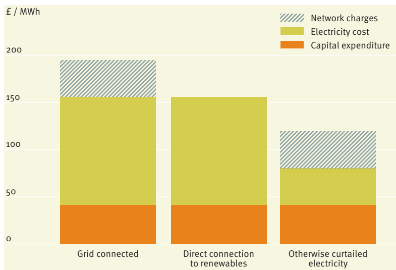
Comparative cost of producing green hydrogen by different methods 38
